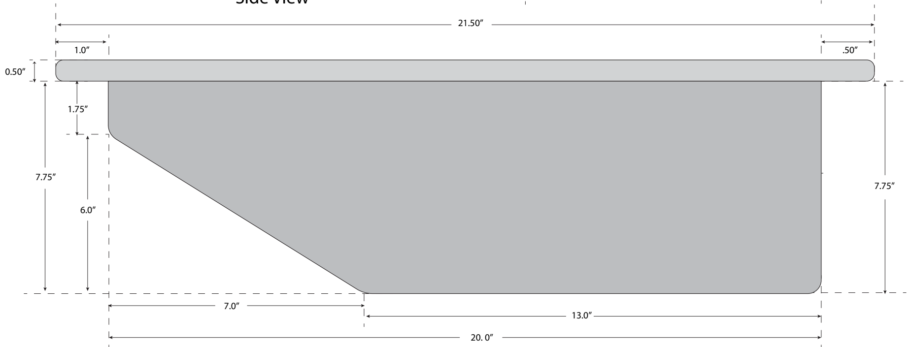
Side View
