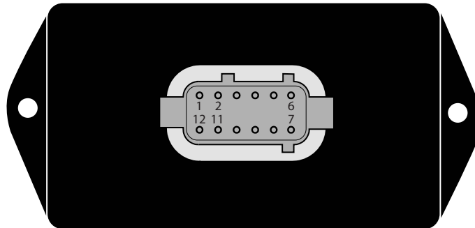
Looking into connector on Tap Shift Module.
