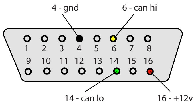
Looking into vehicles OBD II connector.
